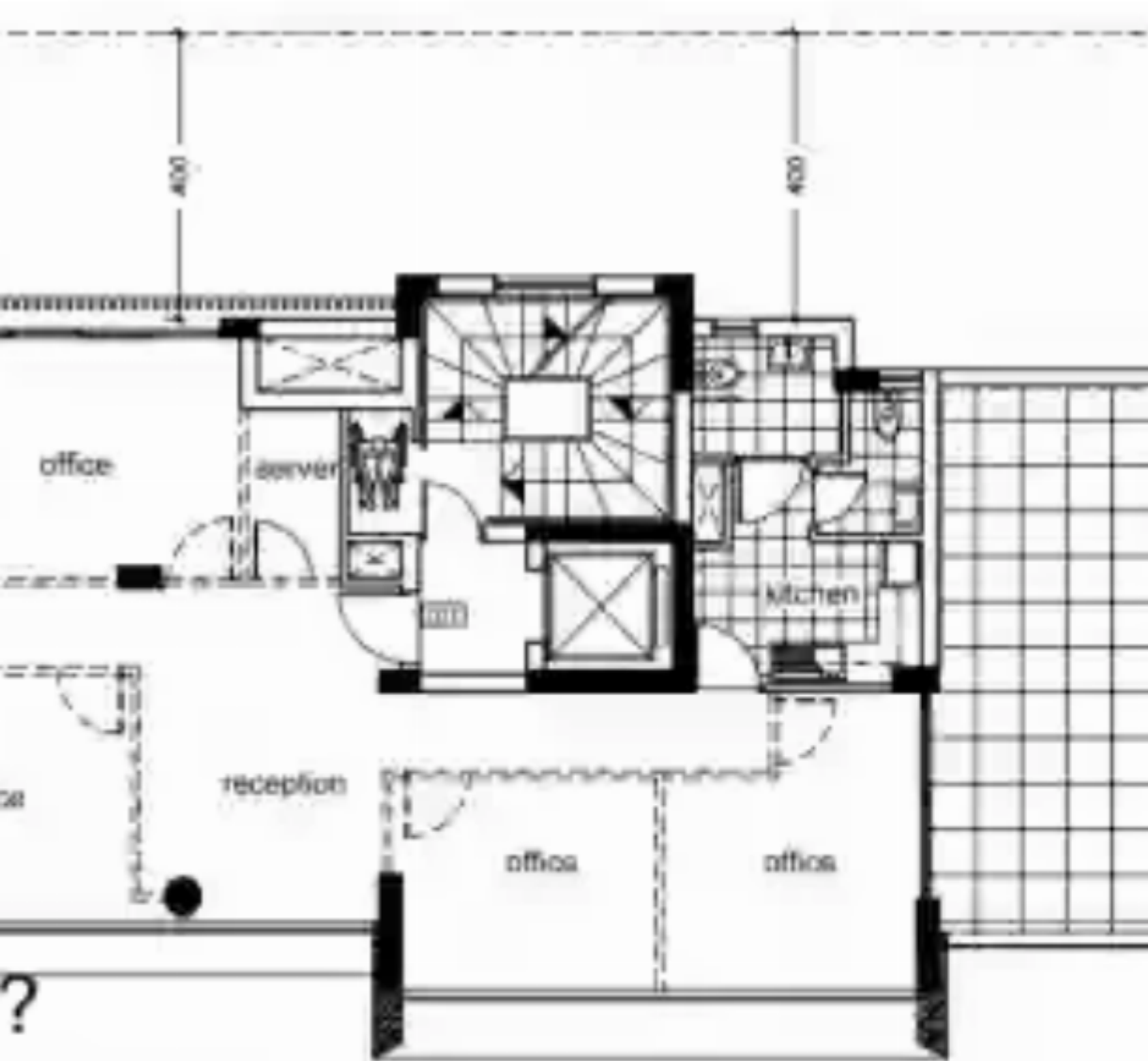
first floor
