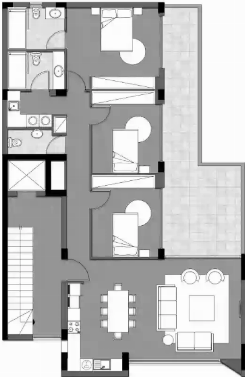
SECOND FLOOR
