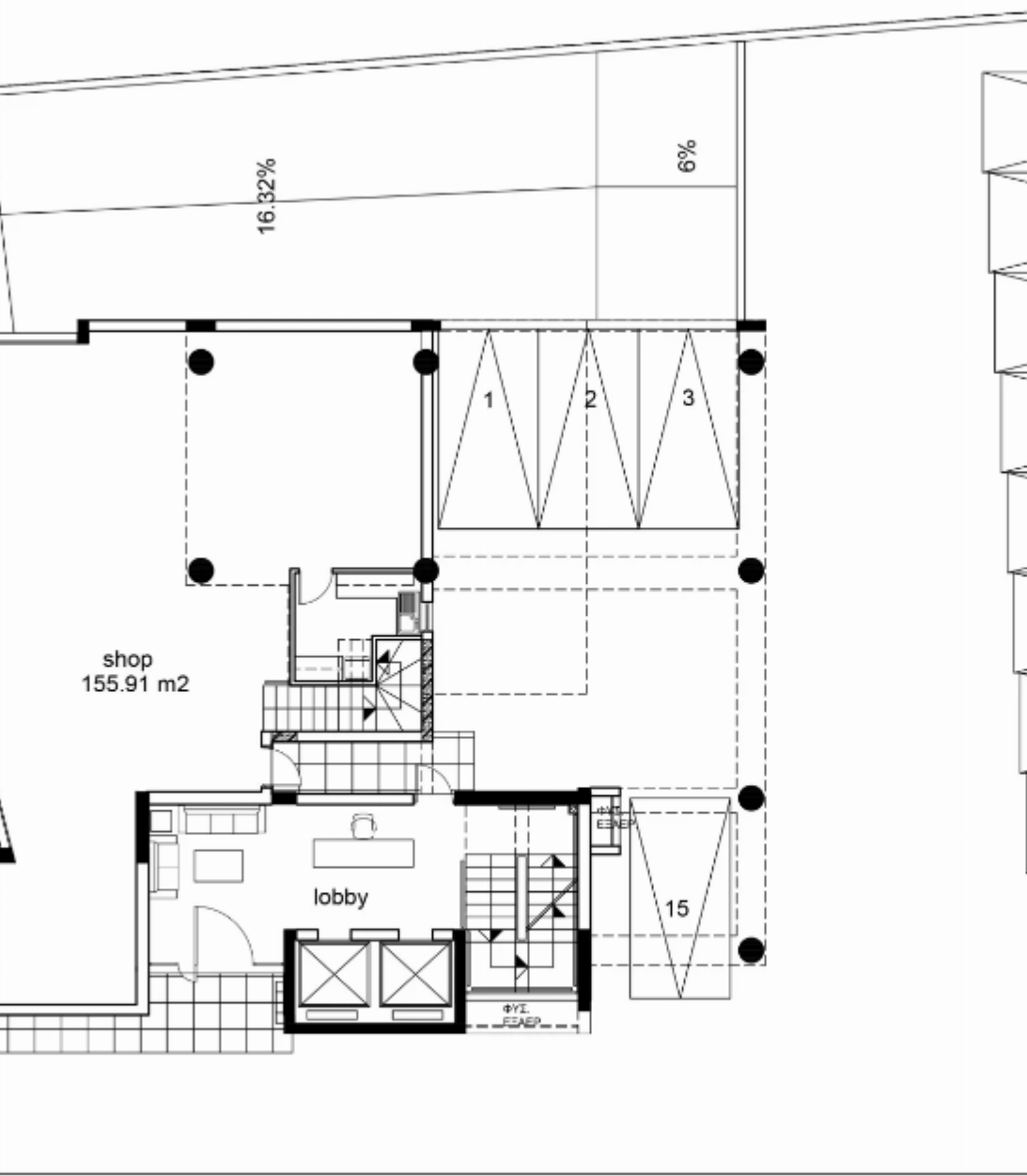
ground floor
